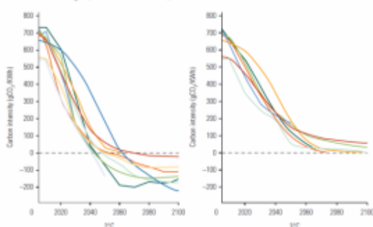
FIGURE 1.4 The Possible Paths to Decarbonizing Electricity (Carbon content of global electricity in two scenarios: on the left-hand side, a stringent GHG concentration target (consistent with 2°C); on the right-hand side, a less stringent GHG concentration target (consistent with 3°C))
